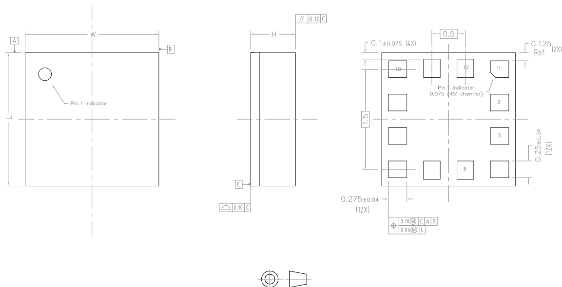
Figure 10. LGA-12L 2.0 x 2.0 x 0.7 mm package outline and mechanical data
