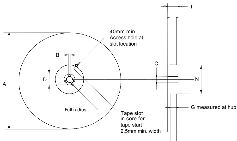
Figure 13. Reel information for carrier tape of LGA-12L package
