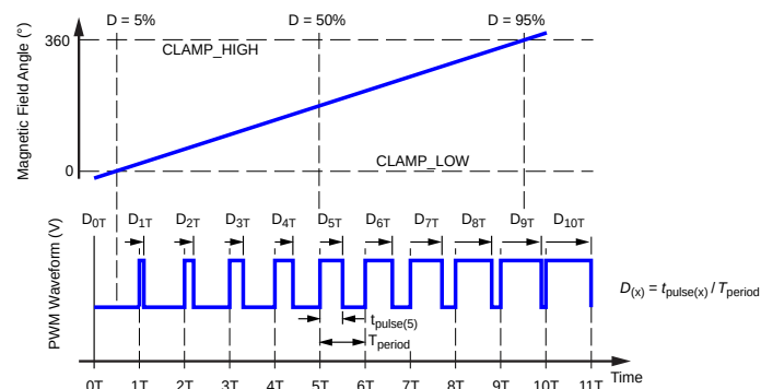
Figure 7: PWM mode outputs a duty-cycle-based waveform that can be read by the external controller as a cumulatively changing continuous voltage.
