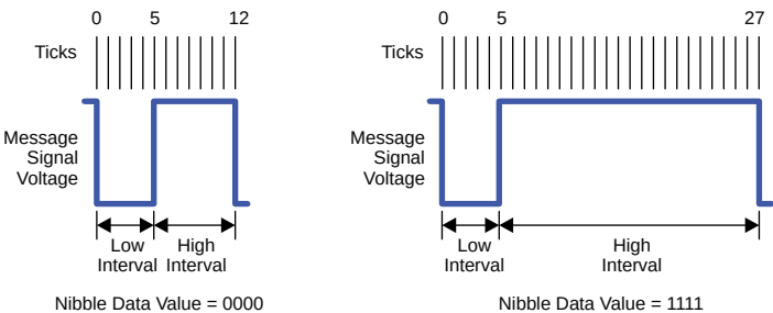
Figure 12: General Value Formation for SENT 0000 (left), 1111 (right)
