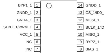
14-Pin TSSOP LE Package Pinouts
