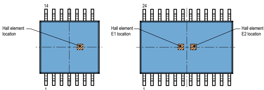
Figure 29: Hall element located off-center within the device body; refer to the Package Outline Drawing for reference dimensions
