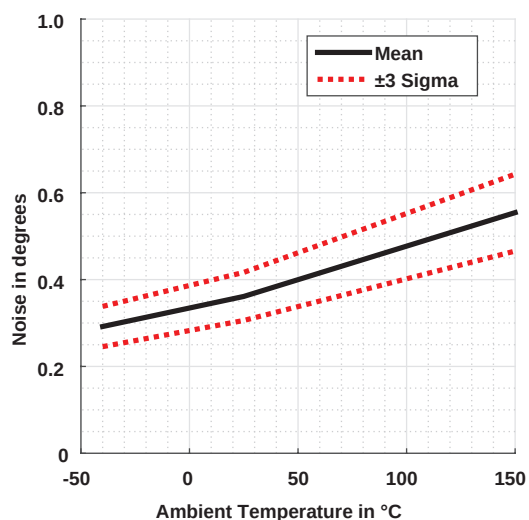
Figure 25: Noise Performance over Temperature (3 \sigma , 300 G)
