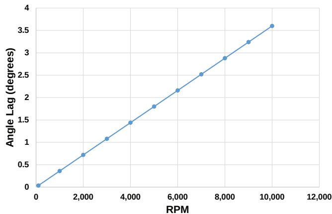
Figure 6: Angle Lag versus RPM, 60 \mu s Response Time
