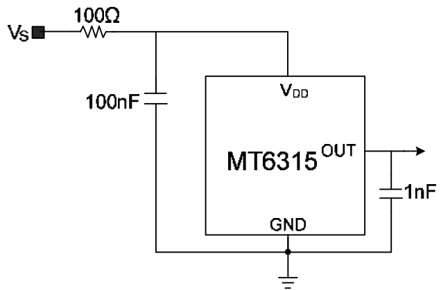
High voltage ( \geq 18\text{V} ), noisy and harsh environment application
