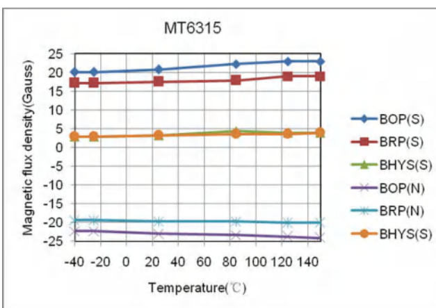
Magnetic Characteristics versus Temperature ( V_{DD}=12\text{V} )
