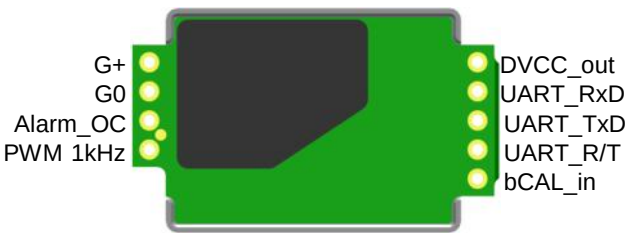
Figure 2. Pin assignment
