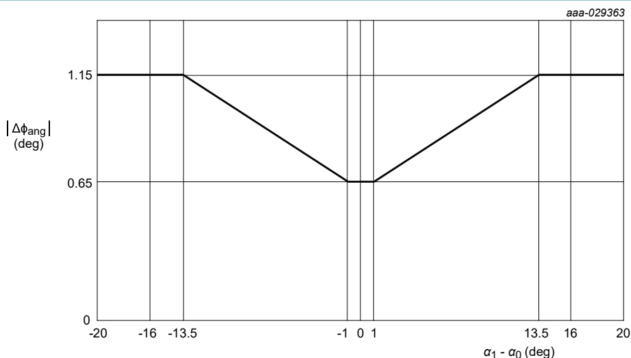
Figure 14. Envelope curve for the magnitude of angular error
