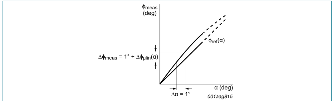
Figure 18. Definition of the microlinearity error
