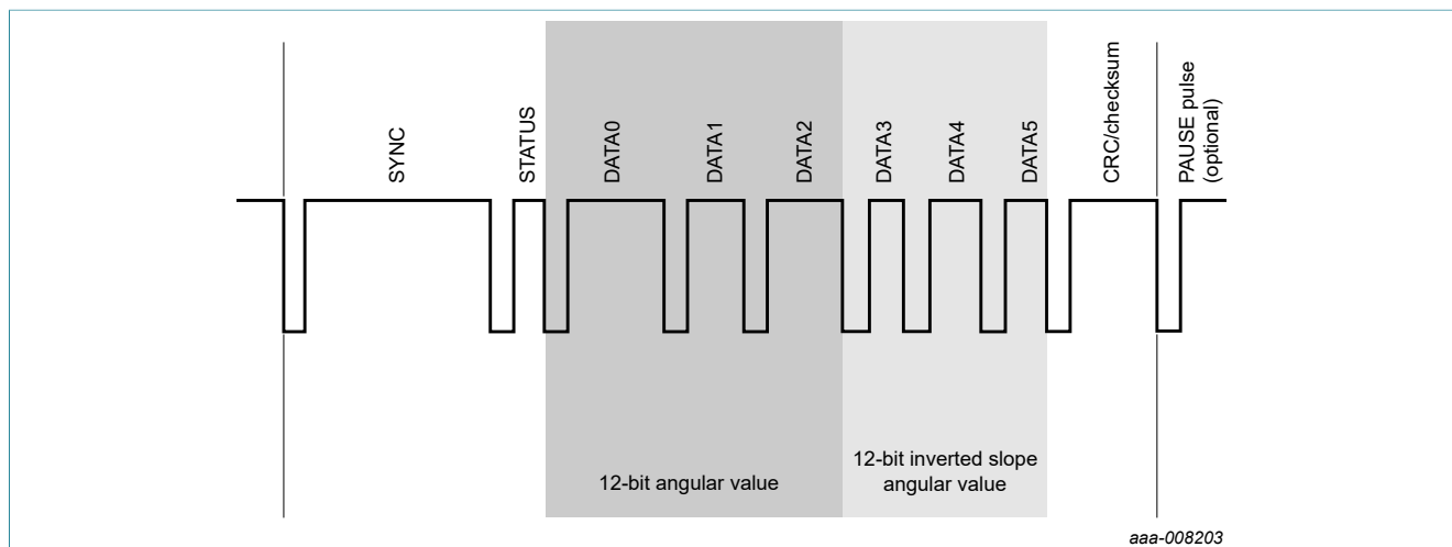
Figure 7. Dual throttle position sensor formats A.1 and H.1
