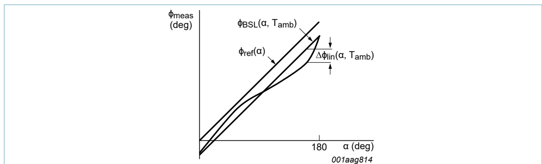
Figure 17. Definition of the linearity error
