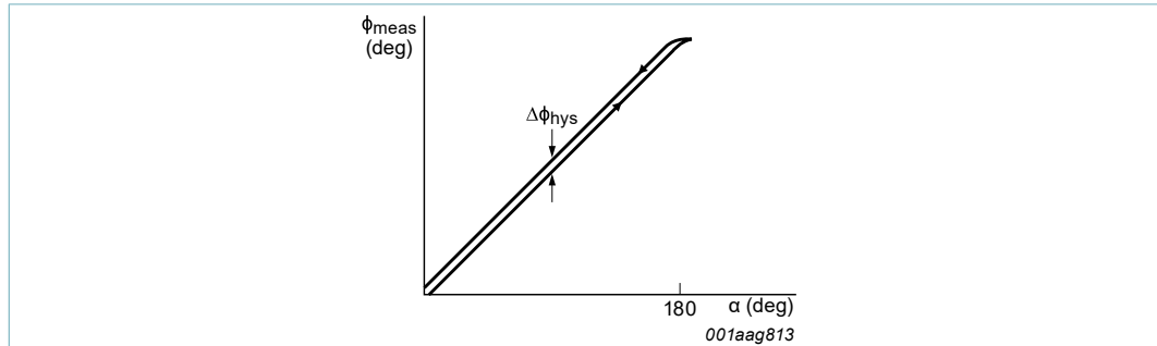
Figure 16. Definition of the hysteresis error
