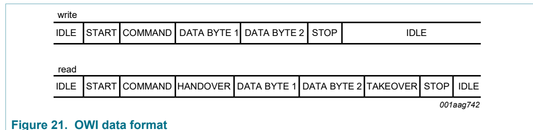
Figure 21. OWI data format
