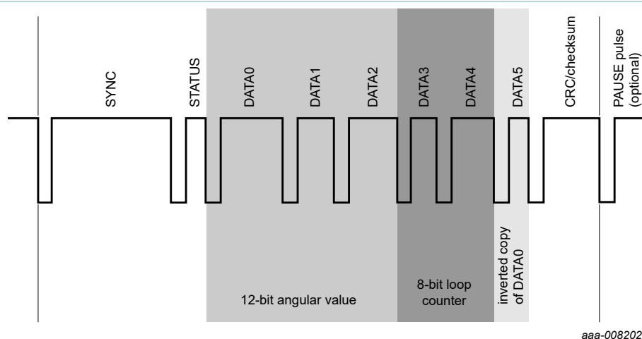
Figure 6. Single secure sensor formats A.3 and H.4
