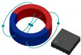
Figure 5: Side-Shaft Mounting
