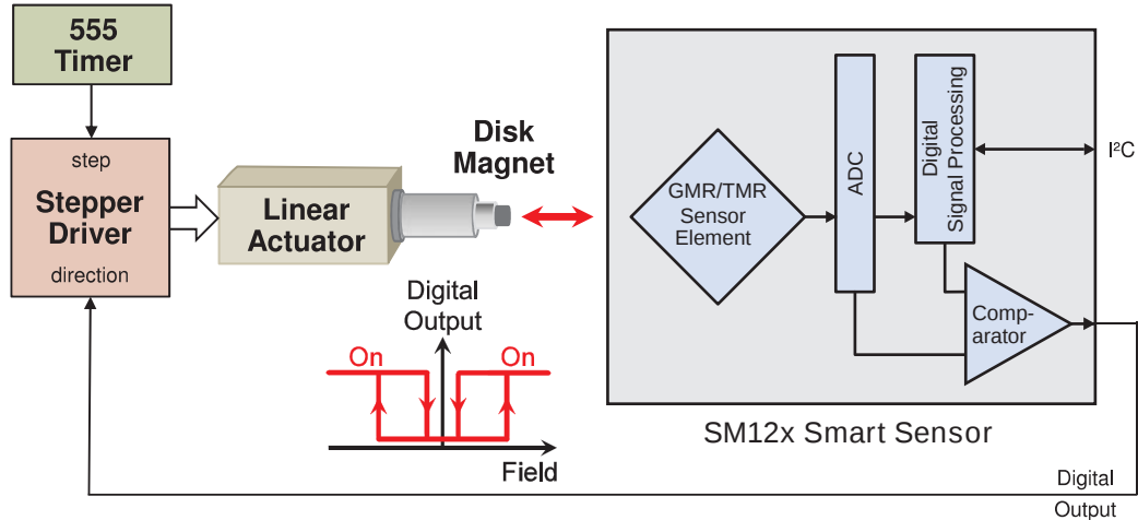
Figure 15. Reciprocating actuator using an SM12x smart sensor.
