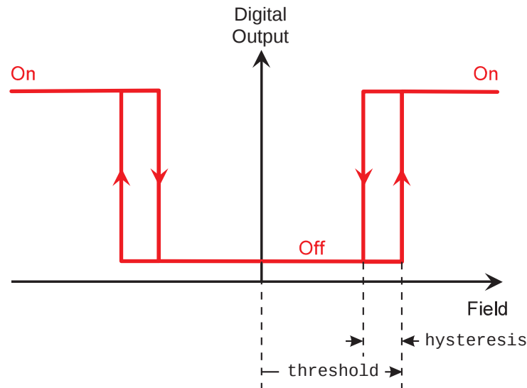
Figure 9. Default Digital Output parameters.
