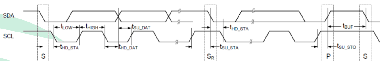
Figure 6: I2C timings
