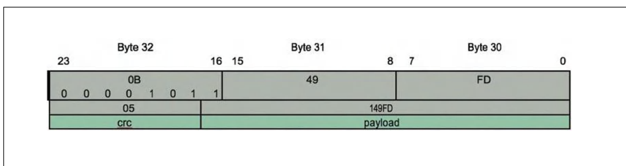
Figure 21: T_VAL Readout
