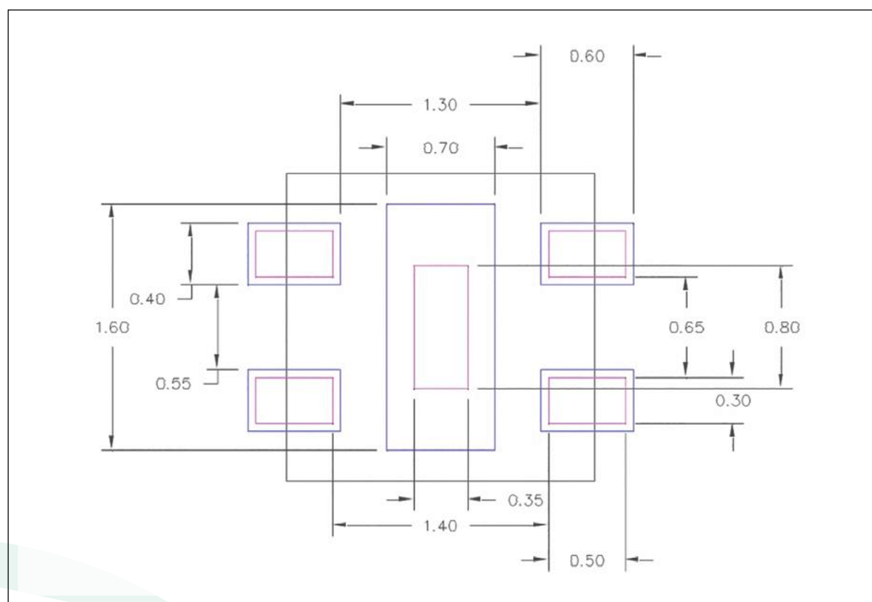
Figure 38: Footprint Design
