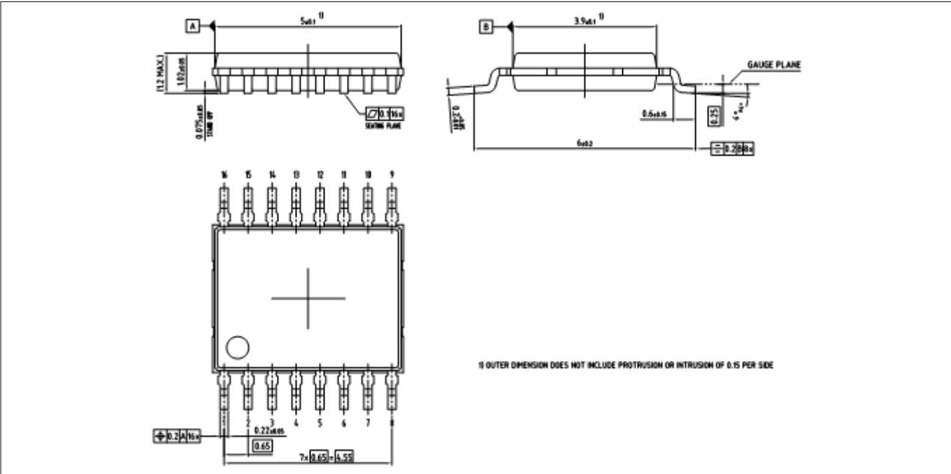
Figure 22 Package dimensions
