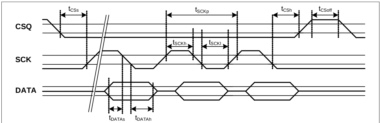
Figure 4-9 SSC timing
