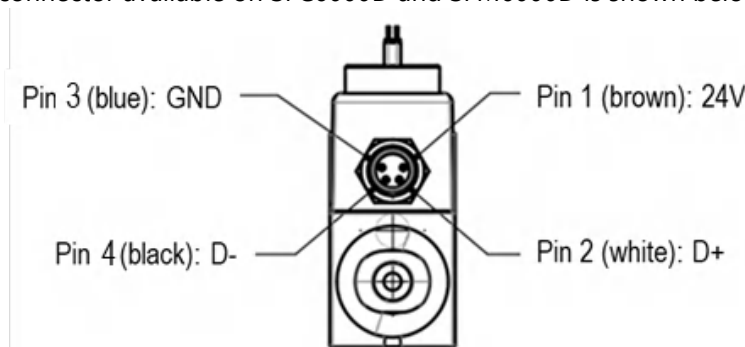
Figure 5. Pinout of M8 connector fitted on SFC6000D and SFM6000D with RS485 interface.
