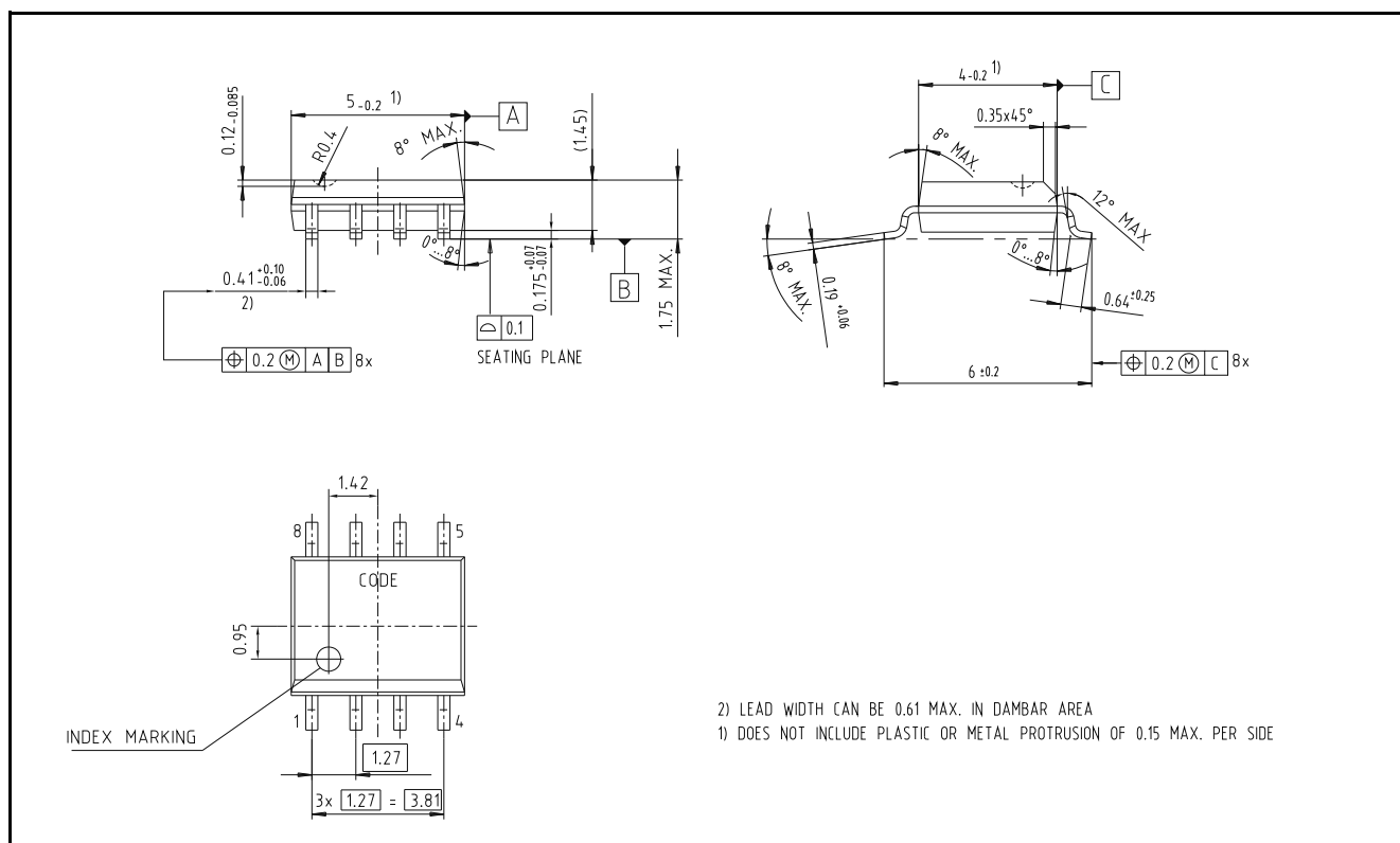
Figure 15 Package dimensions
