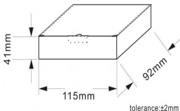
Figure 15. Schematic diagram of packaging
