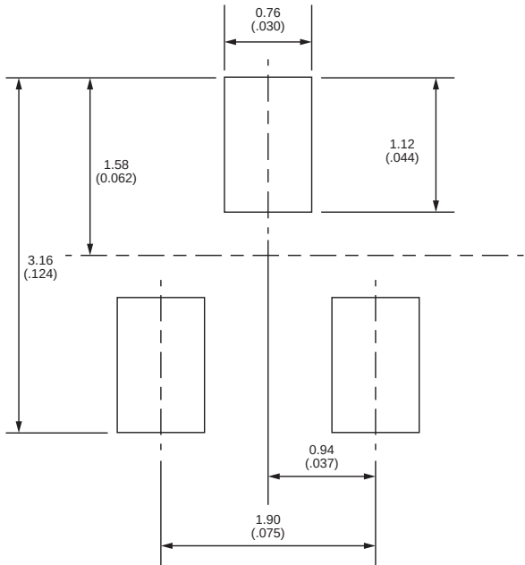
Dimensions in mm (inches) SOT-23-3 Solder Pad Layout
