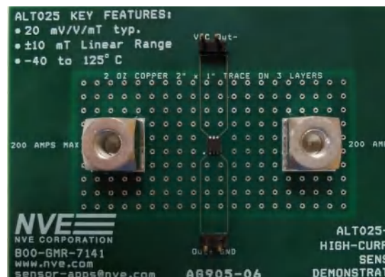
AG905-07E: ALT025-10E High-Current Sensing Evaluation Board.
