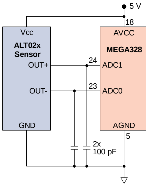
Figure 8. Typical direct microcontroller interface.
