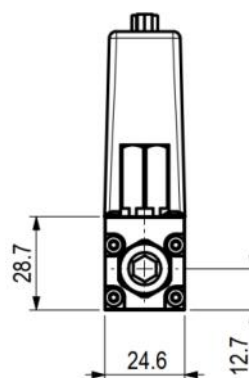
Figure 12: Physical dimensions and mounting information for SFC5500 fitted with a) 6 mm, b) 10 mm Legris connectors. All units are in [mm].
