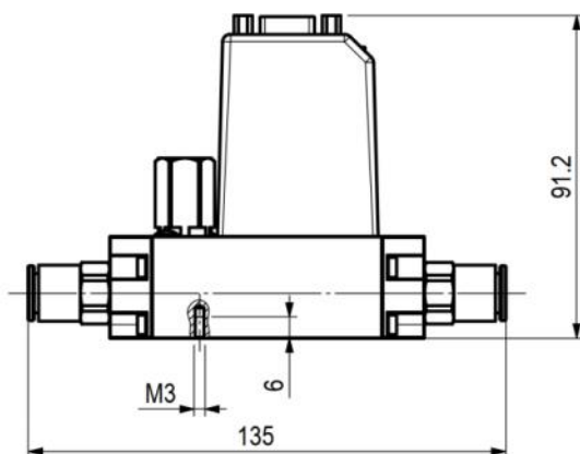
Figure 12: Physical dimensions and mounting information for SFC5500 fitted with a) 6 mm, b) 10 mm Legris connectors. All units are in [mm].
