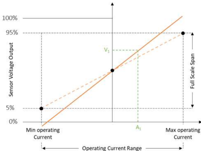
Figure 23: Simple Gain Calibration
