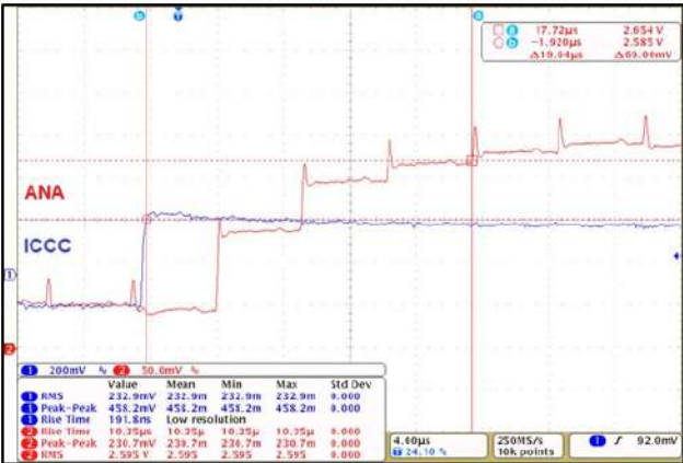
Figure 8: Response Time for CT220
