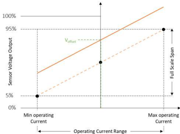
Figure 22: Simple Offset Calibration
