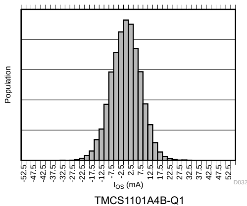
Figure 7-15. Input Offset Current Production Distribution
