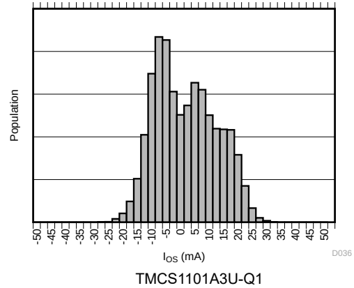
Figure 7-14. Input Offset Current Production Distribution
