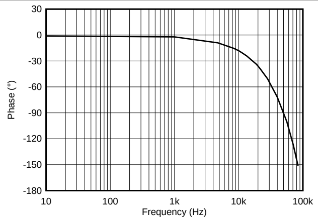
Figure 7-18. Phase vs. Frequency, All Gains
