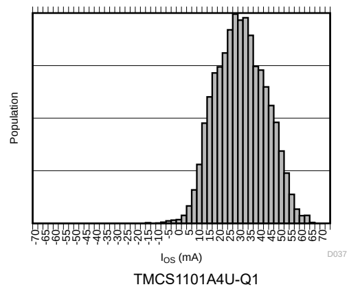
Figure 7-16. Input Offset Current Production Distribution
