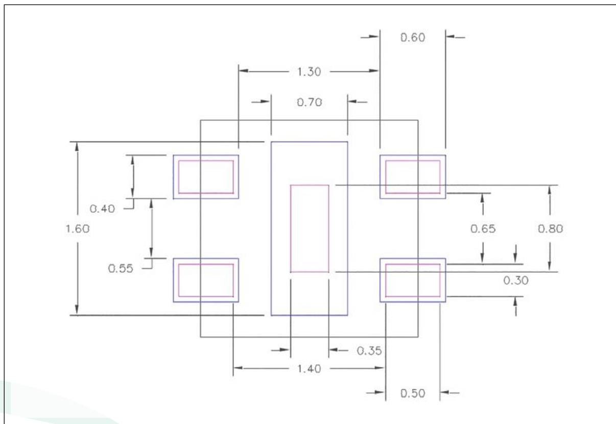
Figure 38: Footprint Design
